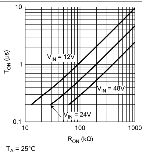
Figure 11. T_{ON} vs R_{ON} , LM3404HV
