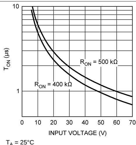
Figure 9. T_{ON} vs V_{IN}
