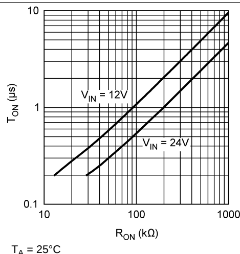
Figure 10. T_{ON} vs R_{ON} , LM3404
