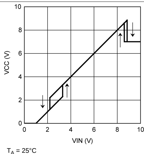
Figure 12. V_{CC} vs V_{IN}
