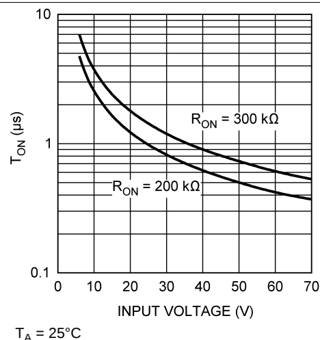
Figure 8. T_{ON} vs V_{IN}
