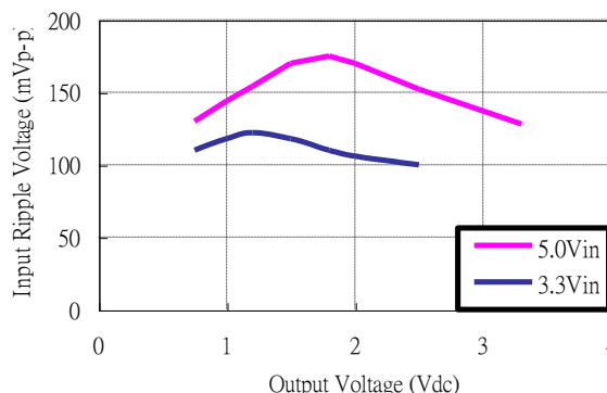
Figure 33: Input voltage ripple for various output models, I_O = 16 A ( C_{IN} = 4 \times 100 \mu F tantalum // 2 x 47 \mu F ceramic)
