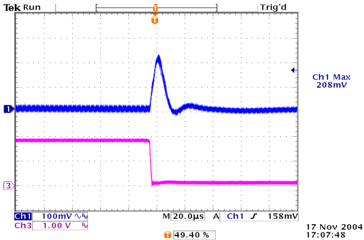
Figure 21: Typical transient response to step load change at 2.5A/\mu S from 100% to 50% of I_o , max at 5Vin, 1.8V out (Cout = ceramic, 10µF tantalum)
