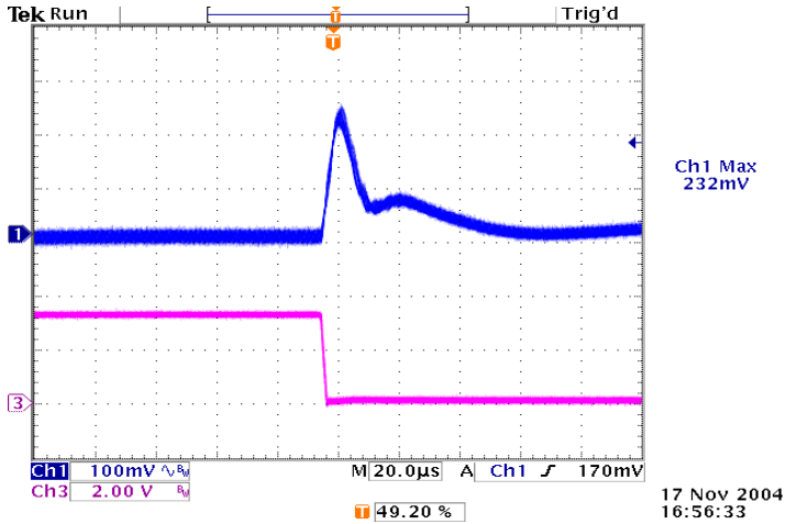
Figure 19: Typical transient response to step load change at 2.5A/\mu S from 100% to 50% of I_o , max at 5Vin, 3.3V out (Cout = ceramic, 10µF tantalum)
