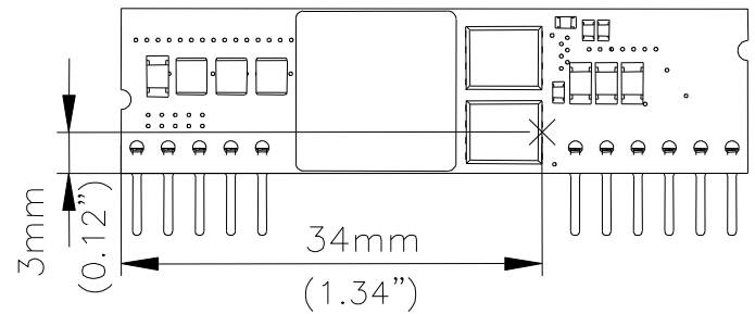
Figure 44: Hot spot temperature measured point
