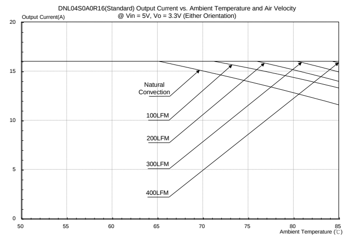
Figure 45: DNL04S0A0R16(Standard) output current vs. ambient temperature and air velocity @Vin=5V, Vo=3.3V(Either Orientation).
