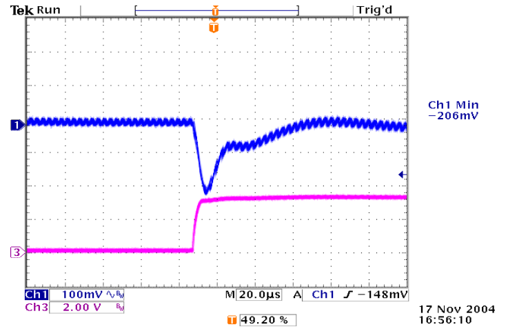
Figure 20: Typical transient response to step load change at 2.5A/\mu S from 50% to 100% of I_o , max at 5Vin, 3.3V out (Cout = ceramic, 10µF tantalum)
