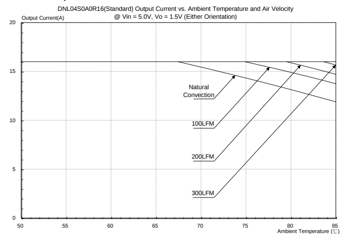
Figure 46: DNL04S0A0R16(Standard) output current vs. ambient temperature and air velocity @Vin=5V, Vo=1.5V(Either Orientation).
