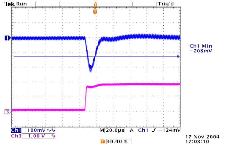
Figure 22: Typical transient response to step load change at 2.5A/\mu S from 50% to 100% of I_o , max at 5Vin, 1.8V out (Cout = ceramic, 10µF tantalum)
