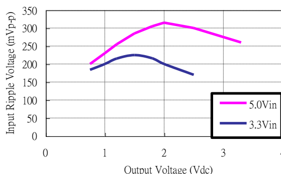
Figure 32: Input voltage ripple for various output models, I_O = 16 A ( C_{IN} = 2 \times 100 \mu F tantalum // 47 \mu F ceramic)
