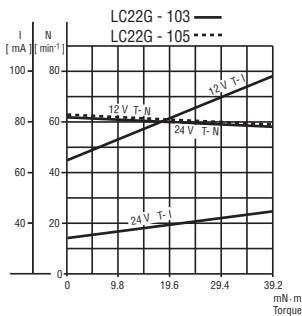
Gear ratio 1/100
