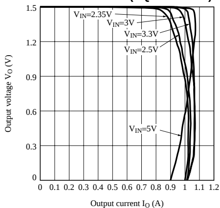
Fig.4 Overcurrent Protection Characteristics (PQ015EZ5MZ)
