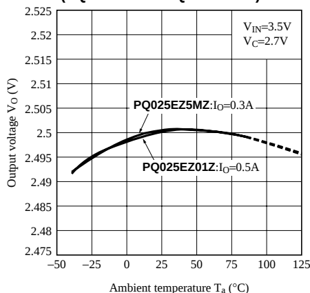
Fig.16 Output Voltage vs. Ambient Temperature (PQ025EZ5MZ/PQ025EZ01Z)
