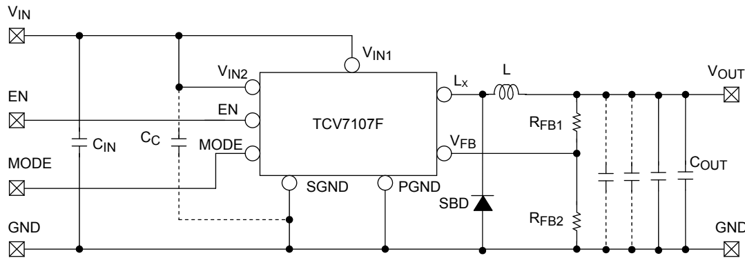
Figure 1 TCV7107F Application Circuit Example
