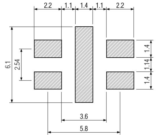
Figure 3) Land Pattern
