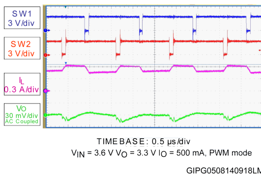
Figure 12. Buck-boost region operation @ I_O = 500\text{ mA}
