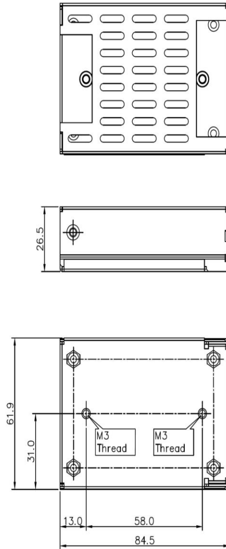
MECHANICAL OUTLINE DIMENSIONS ALL DIMENSIONS ARE IN MM. GEN. TOLERANCE: \pm 1.0 mm
