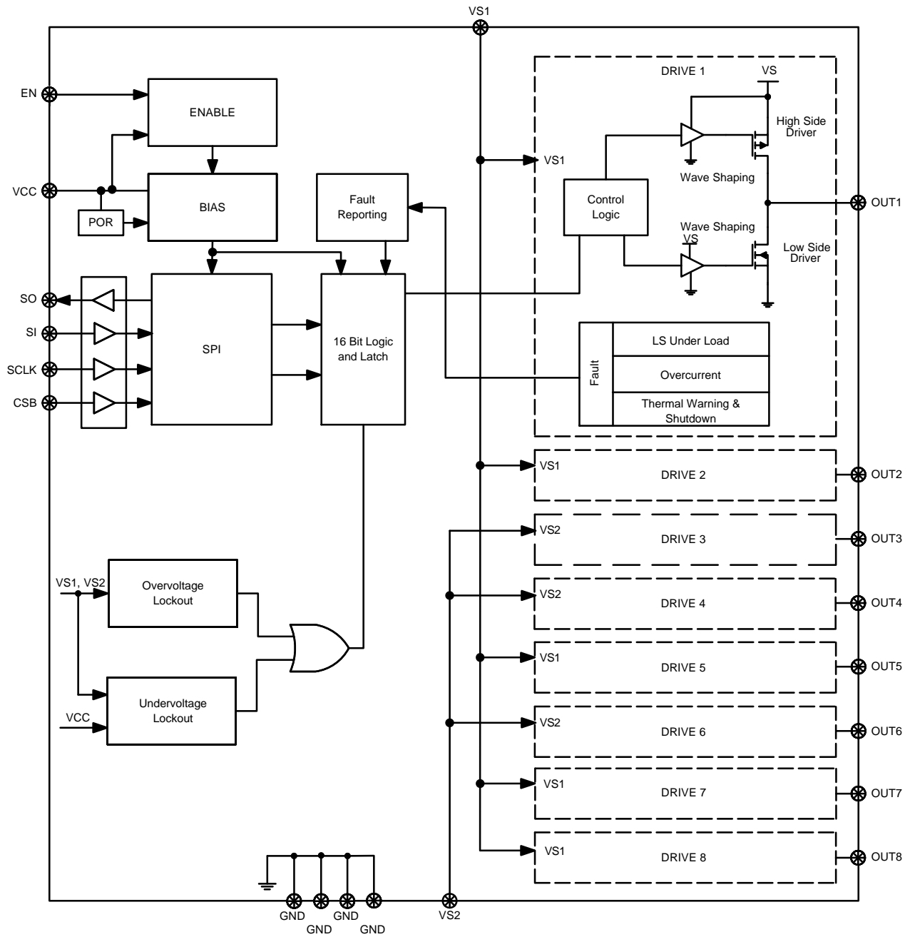
Figure 2. Block Diagram
