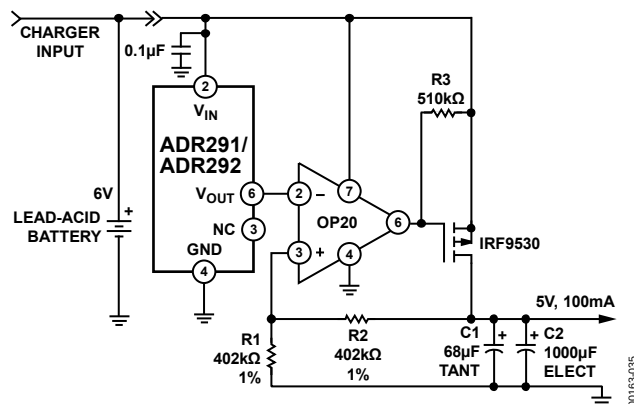
Figure 36. Voltage Regulator for Portable Equipment
