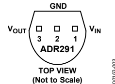
Figure 3. 3-Lead TO-92 (T-3)
