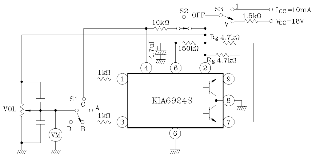
TEST CIRCUIT 1.
