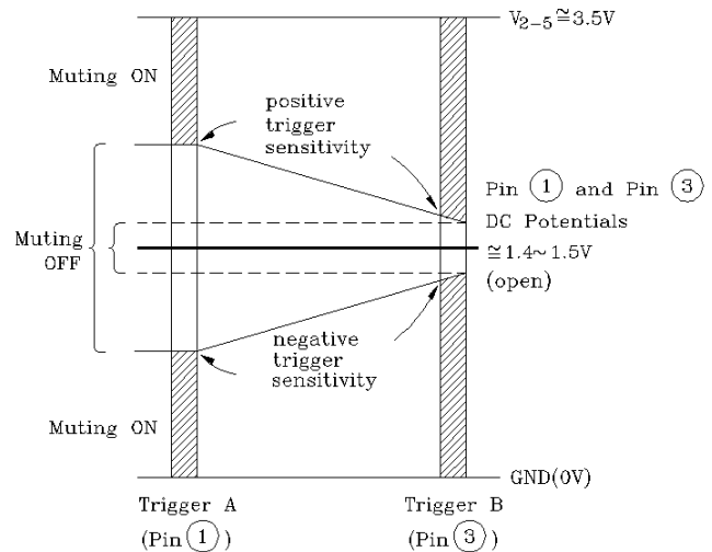
Fig.5 Trigger Level
