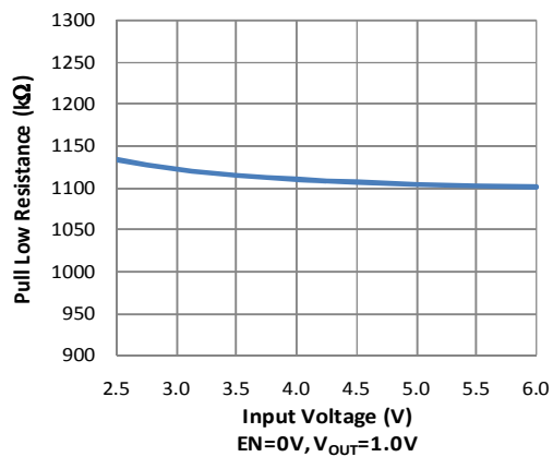
Pull Low Resistance v.s. Input Voltage
