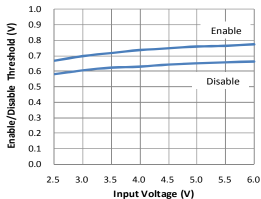
Enable/Disable v.s. Input Voltage
