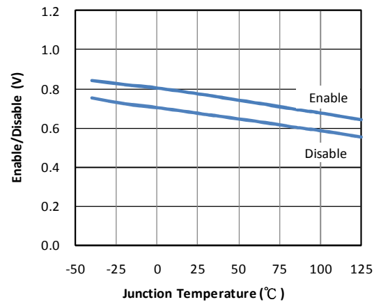
Enable/Disable v.s. Temperature
