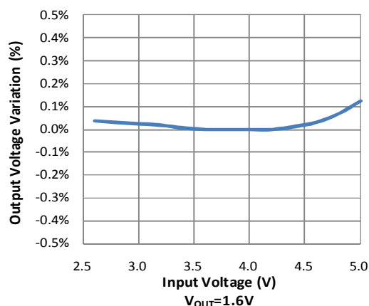
Output Voltage Line Regulation
