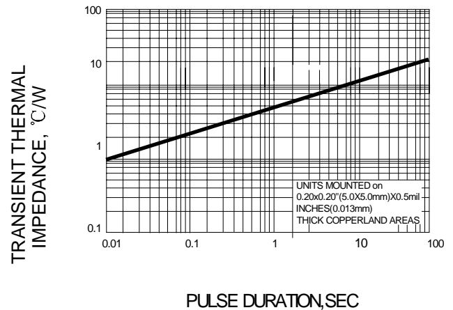
FIG.6-TRANSIENT THERMAL IMPEDANCE
