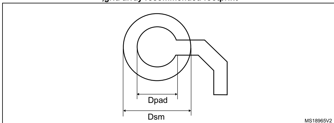
Figure 40. TFBGA64 – 64-ball, 5 x 5 mm, 0.5 mm pitch, thin profile fine pitch ball grid array recommended footprint
