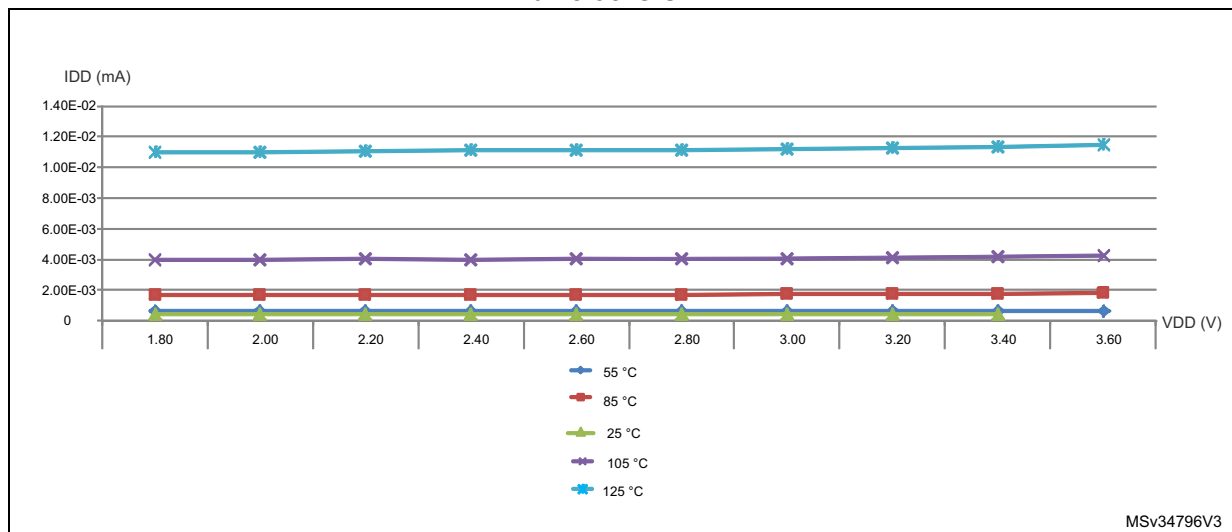
Figure 17. I_{DD} vs V_{DD} , at T_A = 25/55/85/105/125^\circ\text{C} , Stop mode with RTC disabled, all clocks OFF
