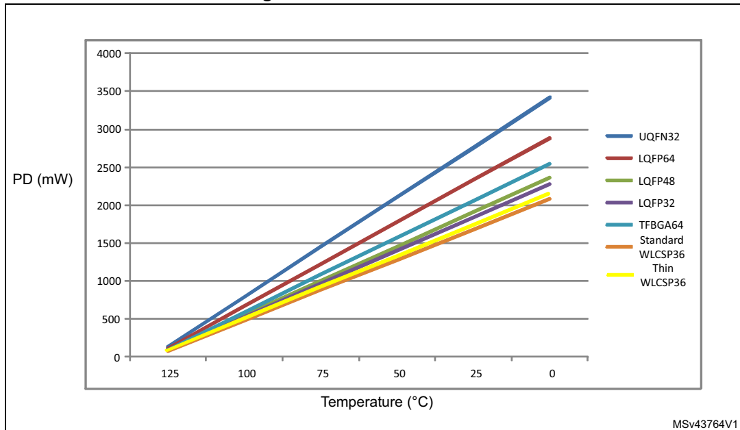
Figure 56. Thermal resistance
