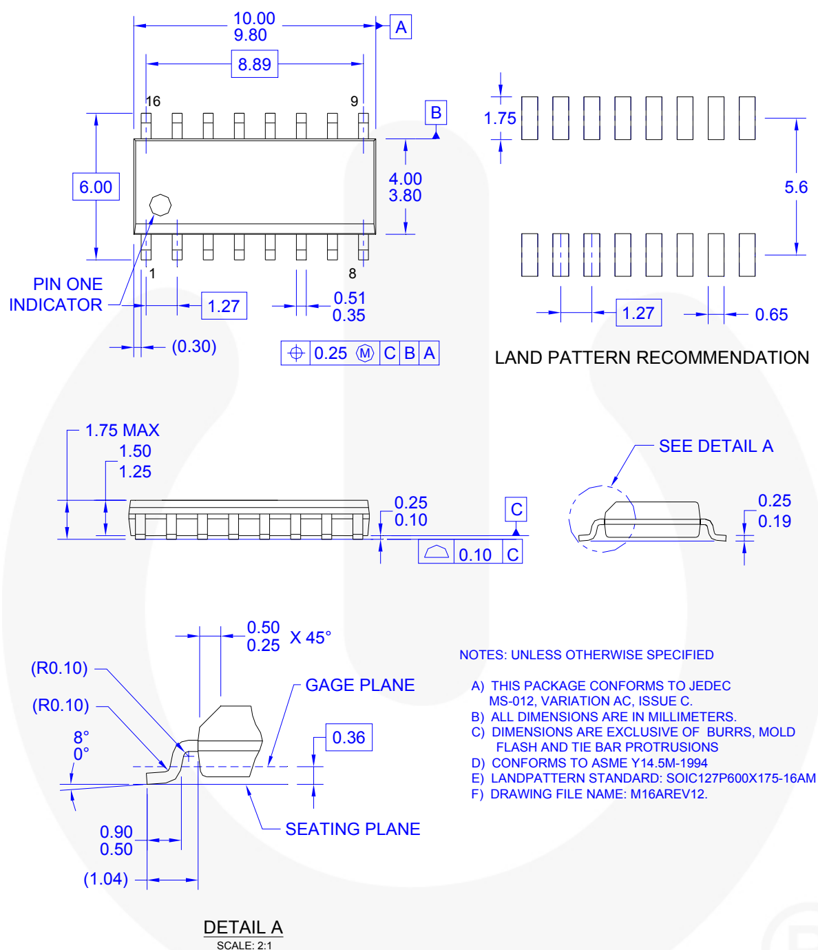
Figure 66. 16-Lead SOIC Package
