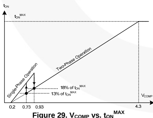
Figure 29. V_{COMP} vs. t_{ON}^{MAX}
