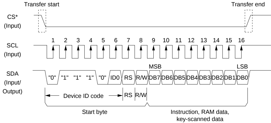
b) Consecutive Data-Transfer Timing through Clock-Synchronized Serial Bus Interface
