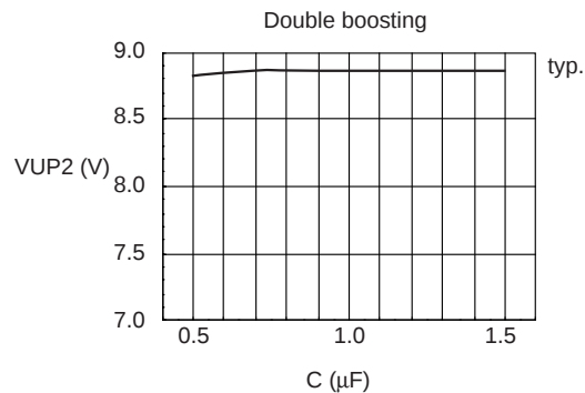
Figure 55 Booster (cont)
