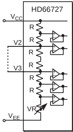
Figure 16 Contrast Adjuster
