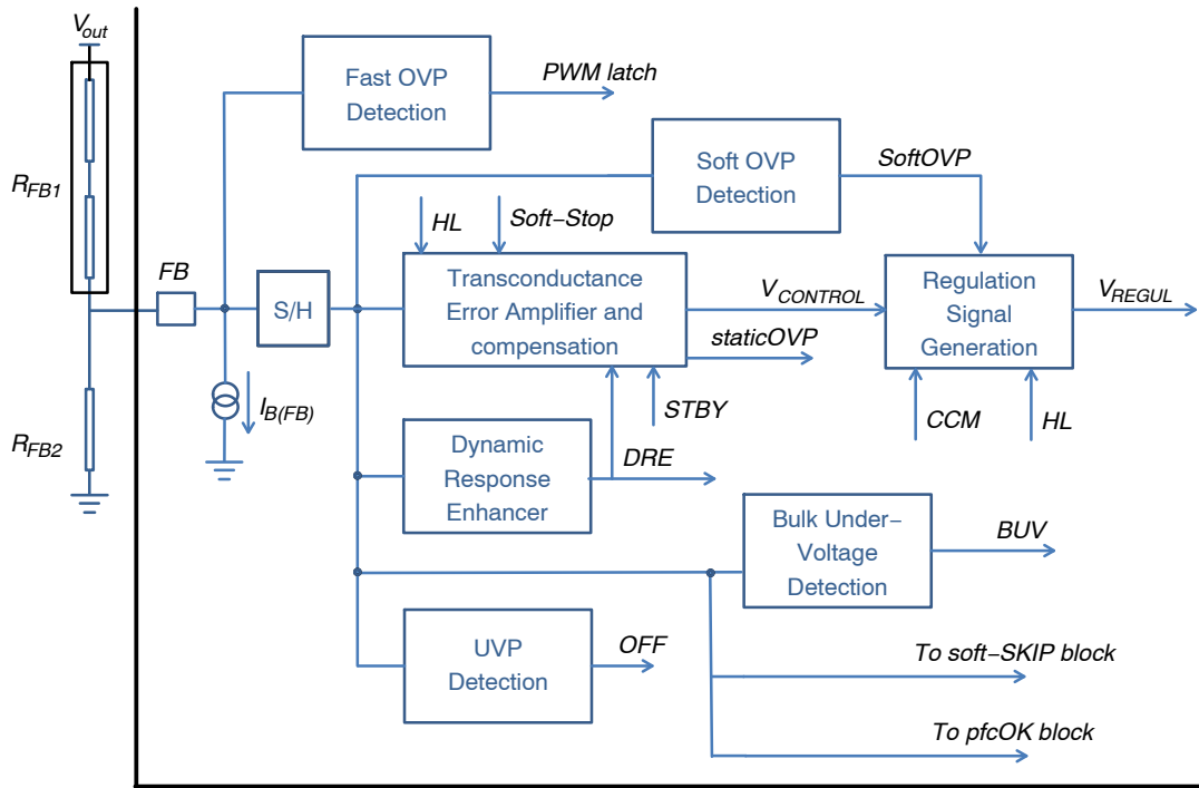
Figure 11. Regulation Circuitry
