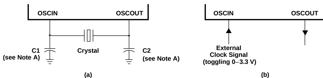
Figure 4. Recommended Crystal/Clock Connection
