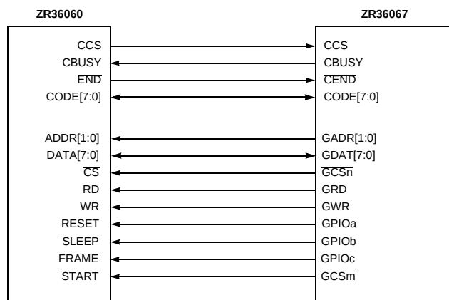
Figure 8. ZR36067 And ZR36050 Host And Code Interfaces
