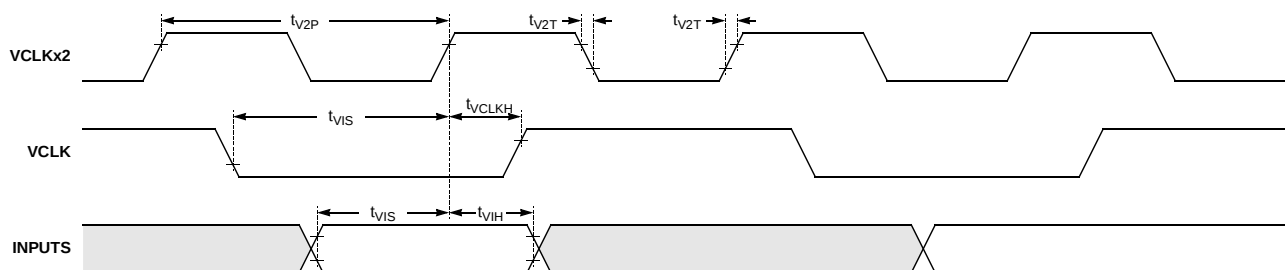
Figure 11. Video Bus Timing
