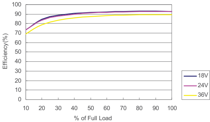
DH24S12-40 Efficiency vs Load Current
