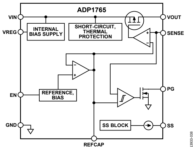
Figure 38. Functional Block Diagram, Fixed Output
