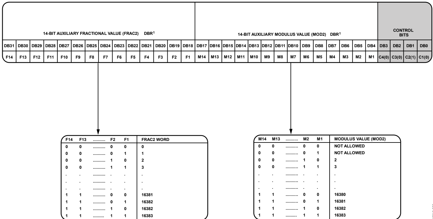
Figure 32. Register 2
