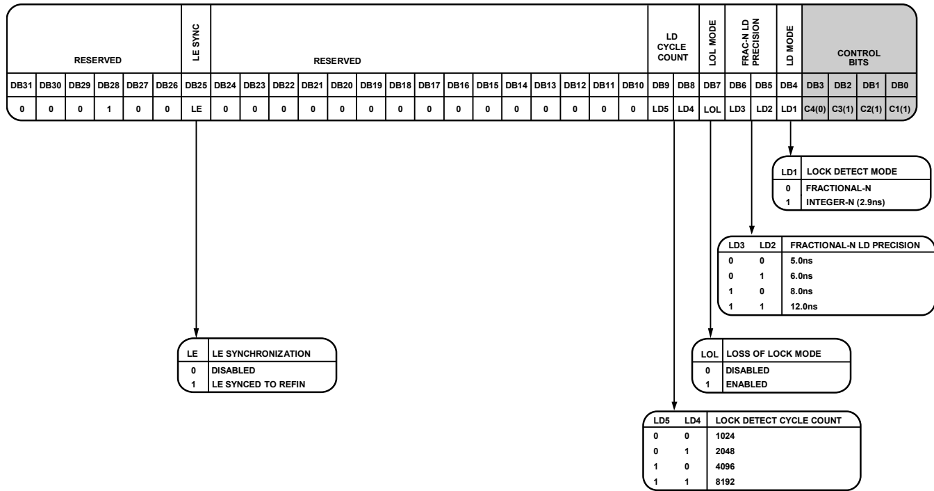
Figure 37. Register 7
