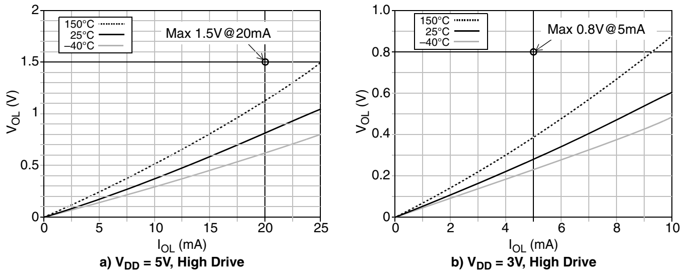
Figure A-1. Typical V_{\text{OL}} vs I_{\text{OL}} , High Drive Strength
