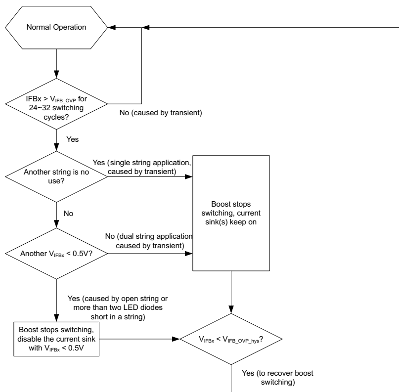
Figure 24. VIFBx OVP Protection Action
