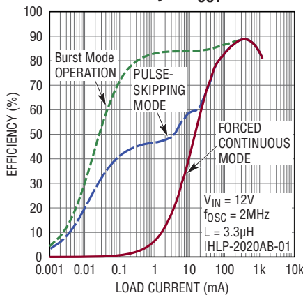
2MHz Efficiency at V_{OUT} = 3.3V
