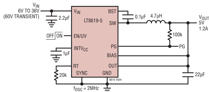
5V 2MHz Step-Down Converter
