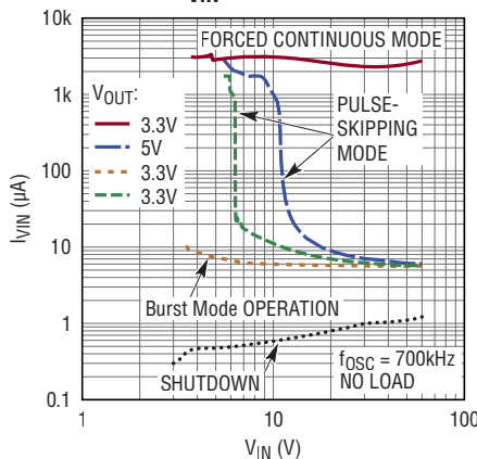
No Load I_{VIN} at 700kHz
