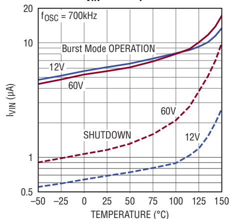
No Load I_{VIN} vs Temperature
