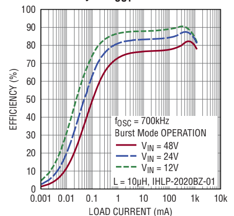
Efficiency at V_{OUT} = 3.3V
