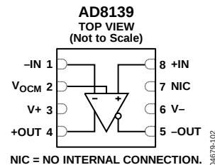
Figure 2. 8-Lead LFCSP
