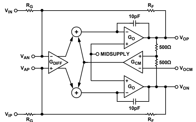
Figure 60. Block Diagram
