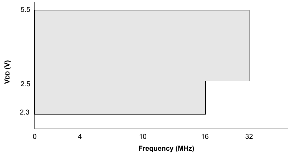
FIGURE 37-1: VOLTAGE FREQUENCY GRAPH, -40^{\circ}\text{C} \leq T_A \leq +125^{\circ}\text{C} , PIC16F15356/75/76/85/86 ONLY
