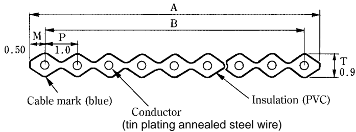
Ribbon Cable
