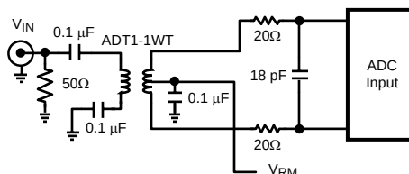
Figure 25. Low Input Frequency Transformer Drive Circuit
