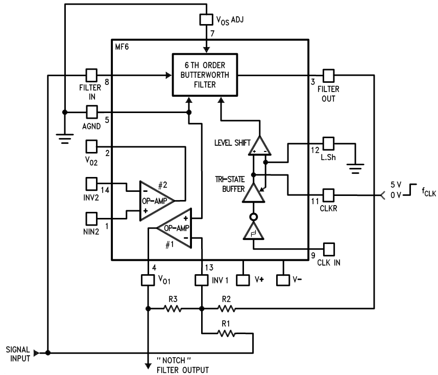
FIGURE 15. "Notch" Filter
