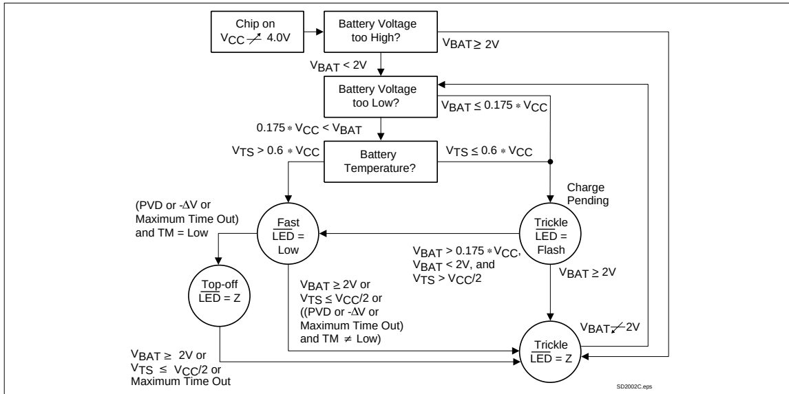
Figure 2. State Diagram
