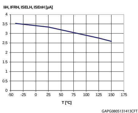
Figure 20: High level logic input current
