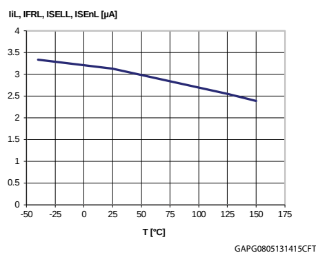
Figure 21: Low level logic input current
