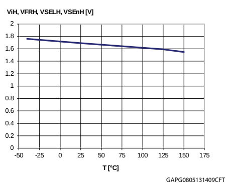
Figure 18: Logic Input high level voltage
