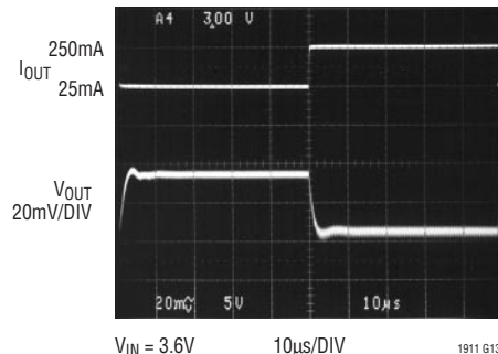
Output Current Transient Response
