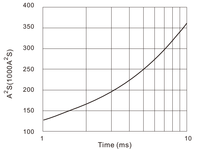
Fig.6 I^2t characteristics
