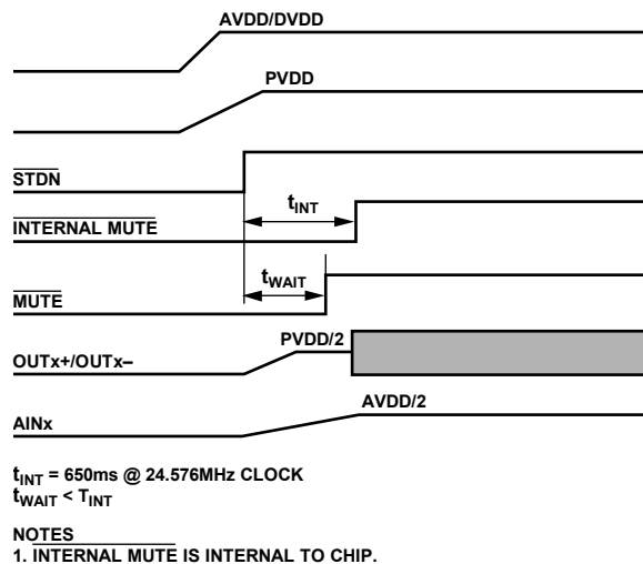
Figure 44. Power-Up Sequence, t_{WAIT} < t_{INT}
