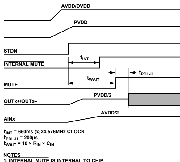
Figure 43. Recommended Power-Up Sequence
