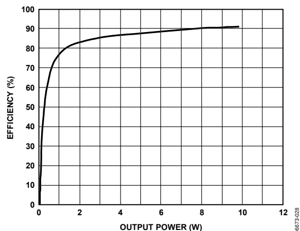
Figure 28. Efficiency vs. Output Power, 12 V, 8 Ω
