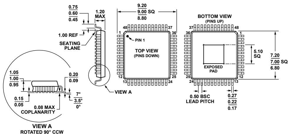
Figure 49. 48-Lead Thin Quad Flat Package, Exposed Pad [TQFP_EP]
