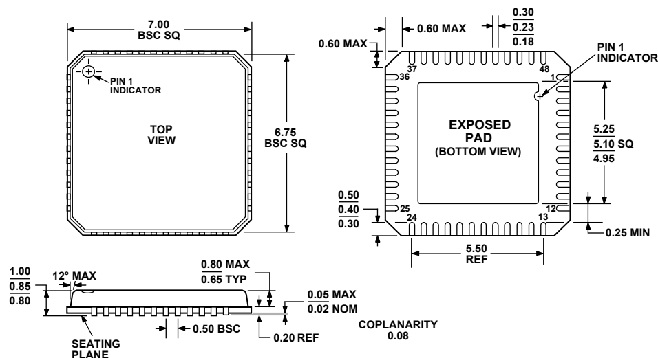
Figure 48. 48-Lead Lead Frame Chip Scale Package [LFCSP_VQ]
