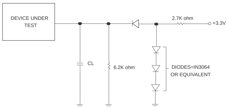
Figure 9. OUTPUT LOADING
