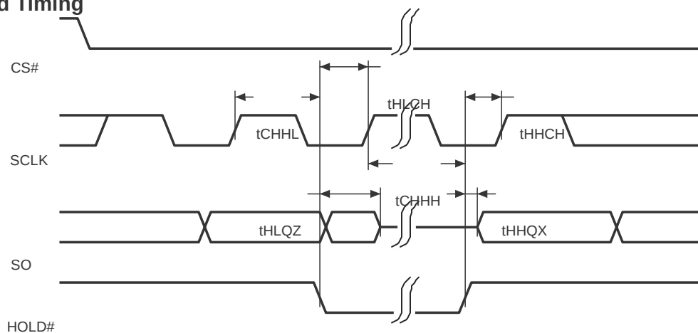
Figure 12. Hold Timing
