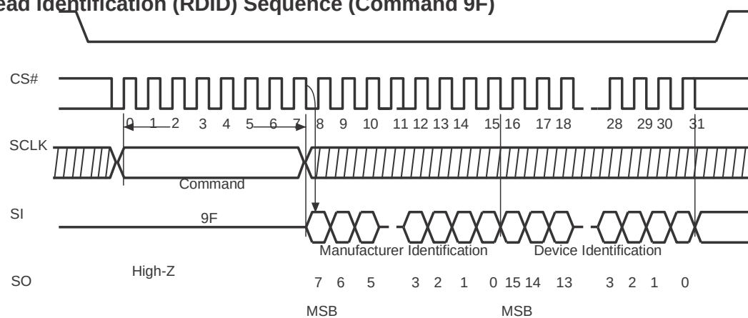
Figure 3. Read Identification (RDID) Sequence (Command 9F)
