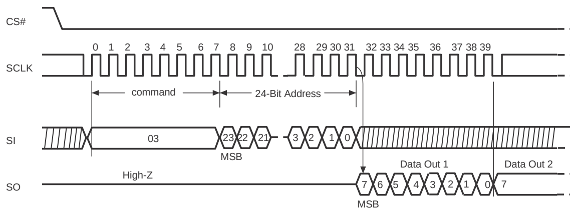
Figure 4. Read Data Bytes (READ) Sequence (Command 03)
