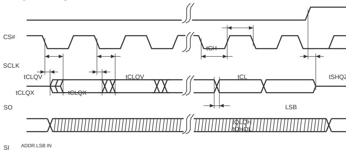
Figure 11. Output Timing
