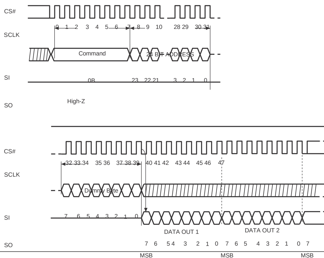
Figure 5. Read at Higher Speed (FAST_READ) Sequence (Command 0B)
