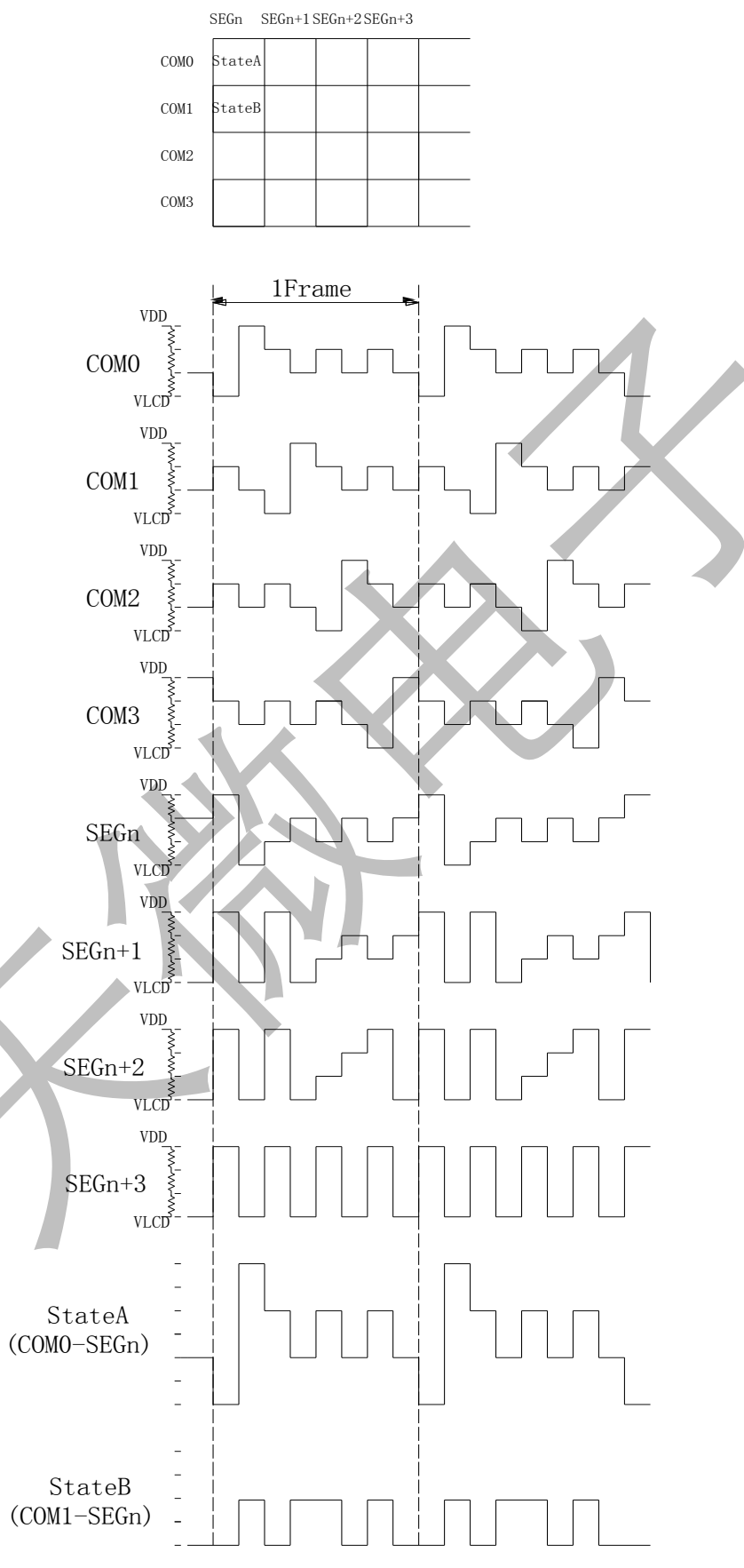
(1) 1/3Bias, Line翻转的液晶驱波形
