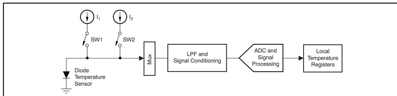
Figure 12. Integrated Local Temperature Sensor
