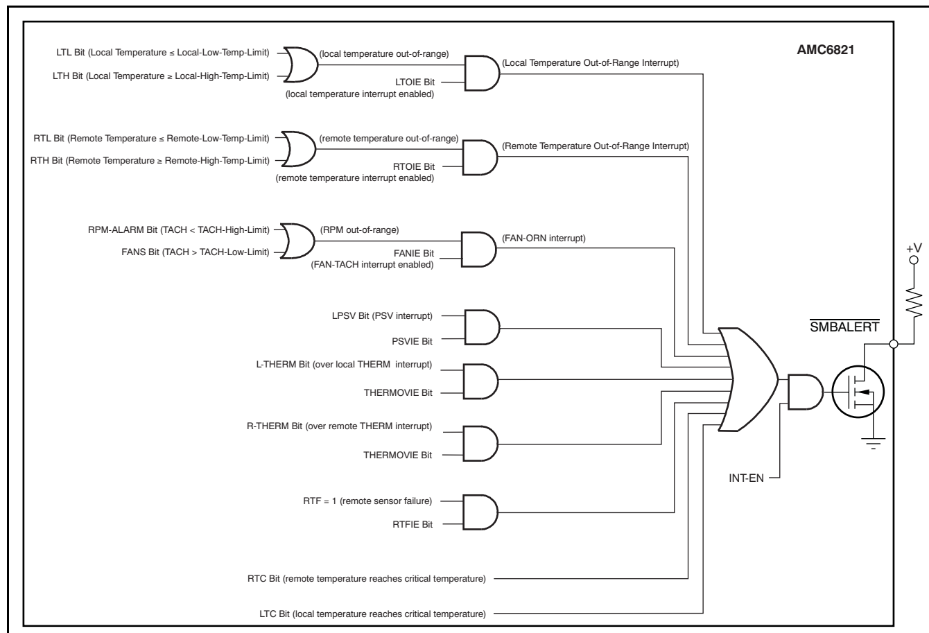
Figure 33. SMBALERT
