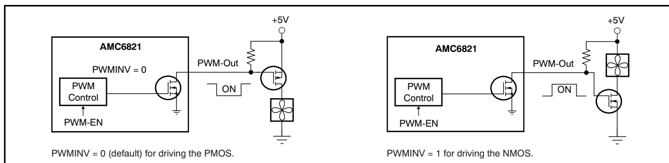
Figure 15. PWM Output
