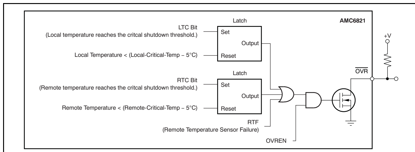
Figure 30. \overline{\text{OVR}} Pin
