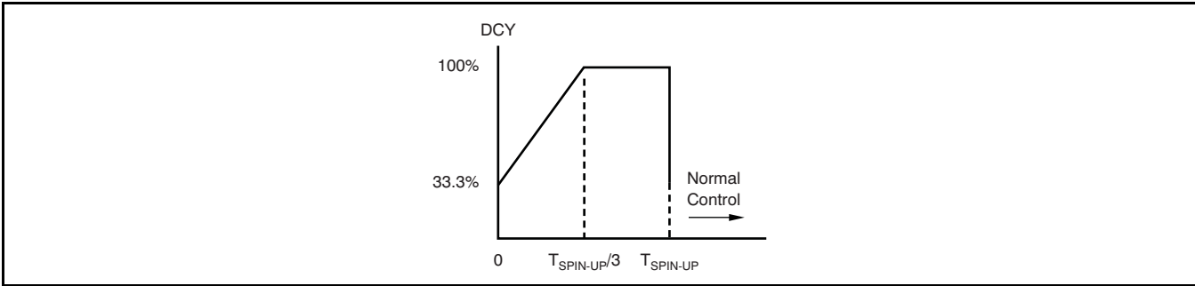
Figure 24. Spin-Up Process
