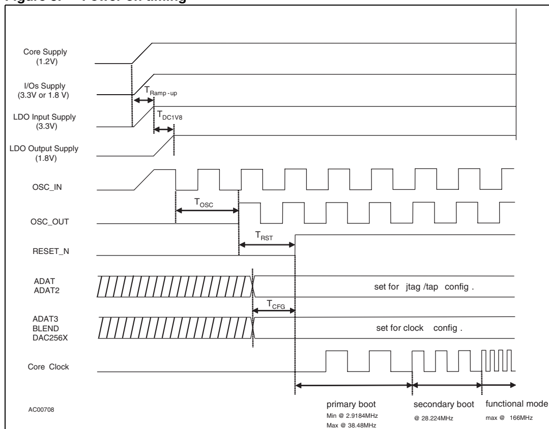
Figure 8. Power on timing
