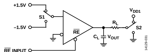
Figure 32. Receiver Enable/Disable
