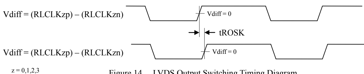
Figure 14. LVDS Output Switching Timing Diagram
