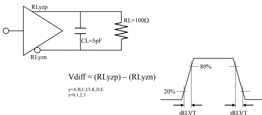
Figure 12. LVDS Output Switching Timing Diagram and Test Circuit
