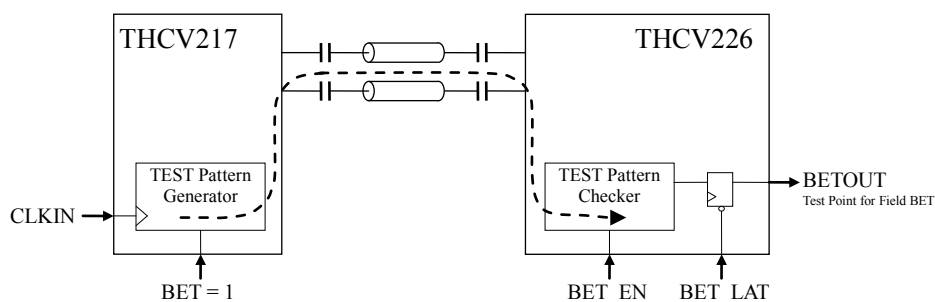
Figure 7. Field BET Configuration
