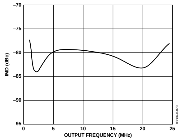
Figure 51. AD9861 Tx Path Dual-Tone (0.5 MHz Spacing) IMD vs. Output Frequency of Tx Path, with 2 mA Full-Scale Output into 600 \Omega Differential Load
