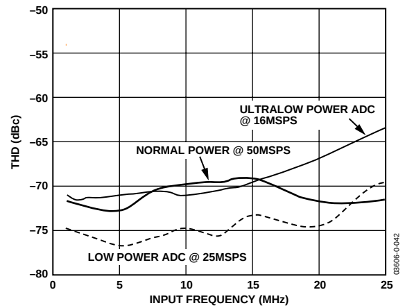
Figure 15. AD9861-50 Rx Path at 50 MSPS, 10 MHz Input Tone THD Performance vs. Input Frequency
