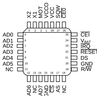
DS14285Q 28-Pin PLCC
