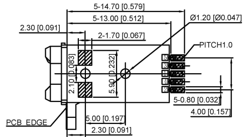
RECOMMENDED P.C.B LAYOUT TOP VIEW (TOLRANCE:±0.05)
