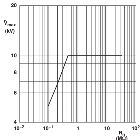
Maximum allowed peak pulse voltage in accordance with "IEC 60065 chapter 14.1"; 50 discharges from a 1 nF capacitor charged to \hat{V}_{max} ; 12 discharges/minute (drift \Delta R/R \leq 2\% ).
