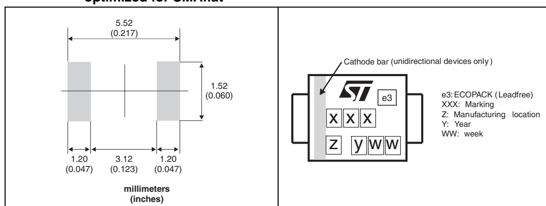
Figure 11. SMAflat footprint dimensions optimized for SMAflat (1) Figure 12. Marking information
