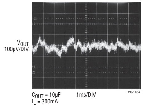
LT1962-5 10Hz to 100kHz Output Noise ( C_{\text{BYP}} = 1000\text{pF} )
