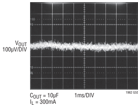
LT1962-5 10Hz to 100kHz Output Noise ( C_{\text{BYP}} = 0.01\mu\text{F} )
