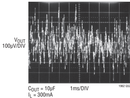
LT1962-5 10Hz to 100kHz Output Noise ( C_{\text{BYP}} = 0 )
