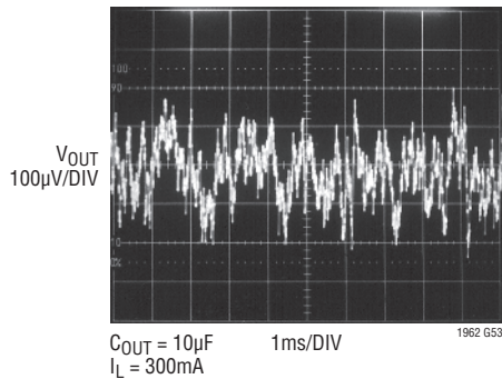
LT1962-5 10Hz to 100kHz Output Noise ( C_{\text{BYP}} = 100\text{pF} )
