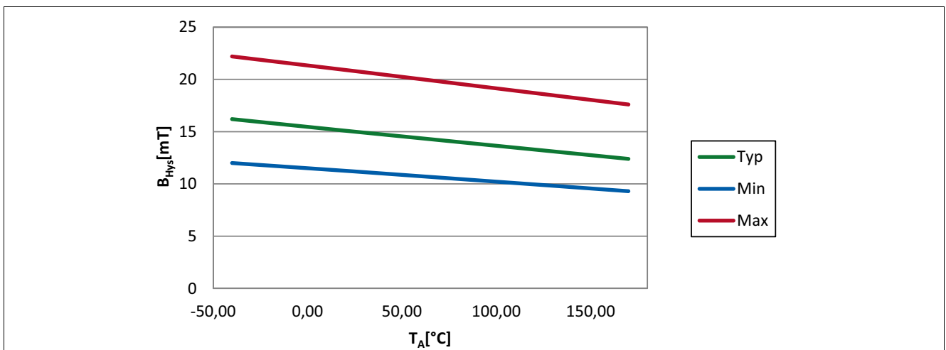
Figure 5-3 Hysteresis (B Hys ) of the TLE4961-3K over Temperature
