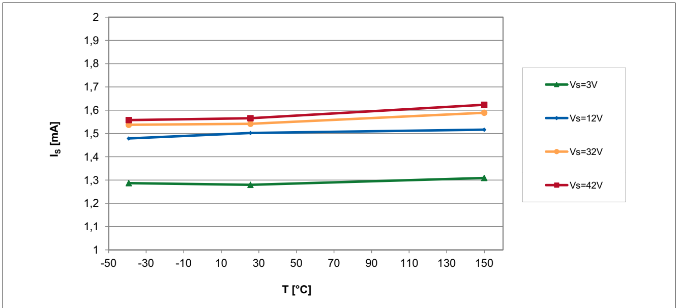
Figure 6-3 Supply Current of the TLE4961-3K over Temperature
