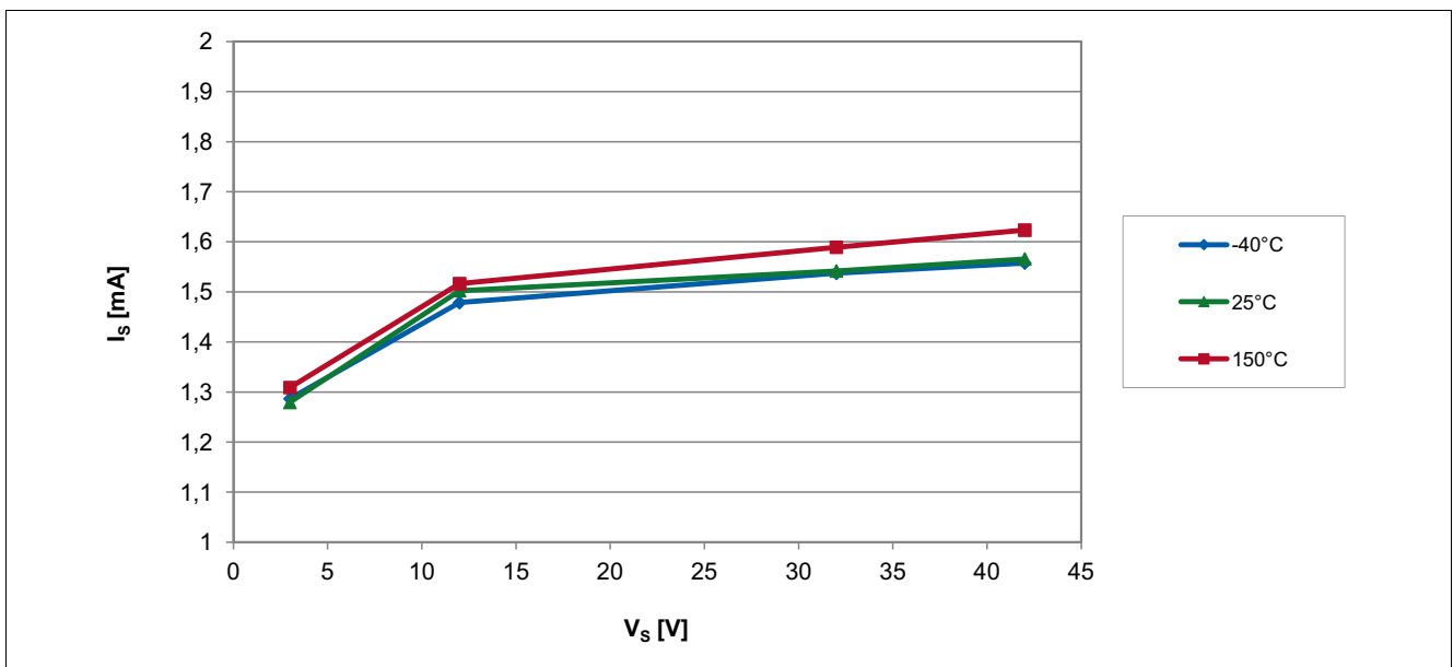
Figure 6-4 Supply Current of the TLE4961-3K over Supply Voltage
