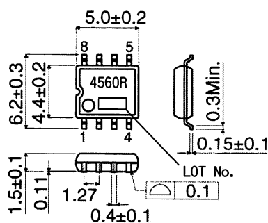
BA4560RF (SOP8) (Unit:[mm])
