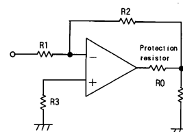
Fig.2 The example of protection resistor
