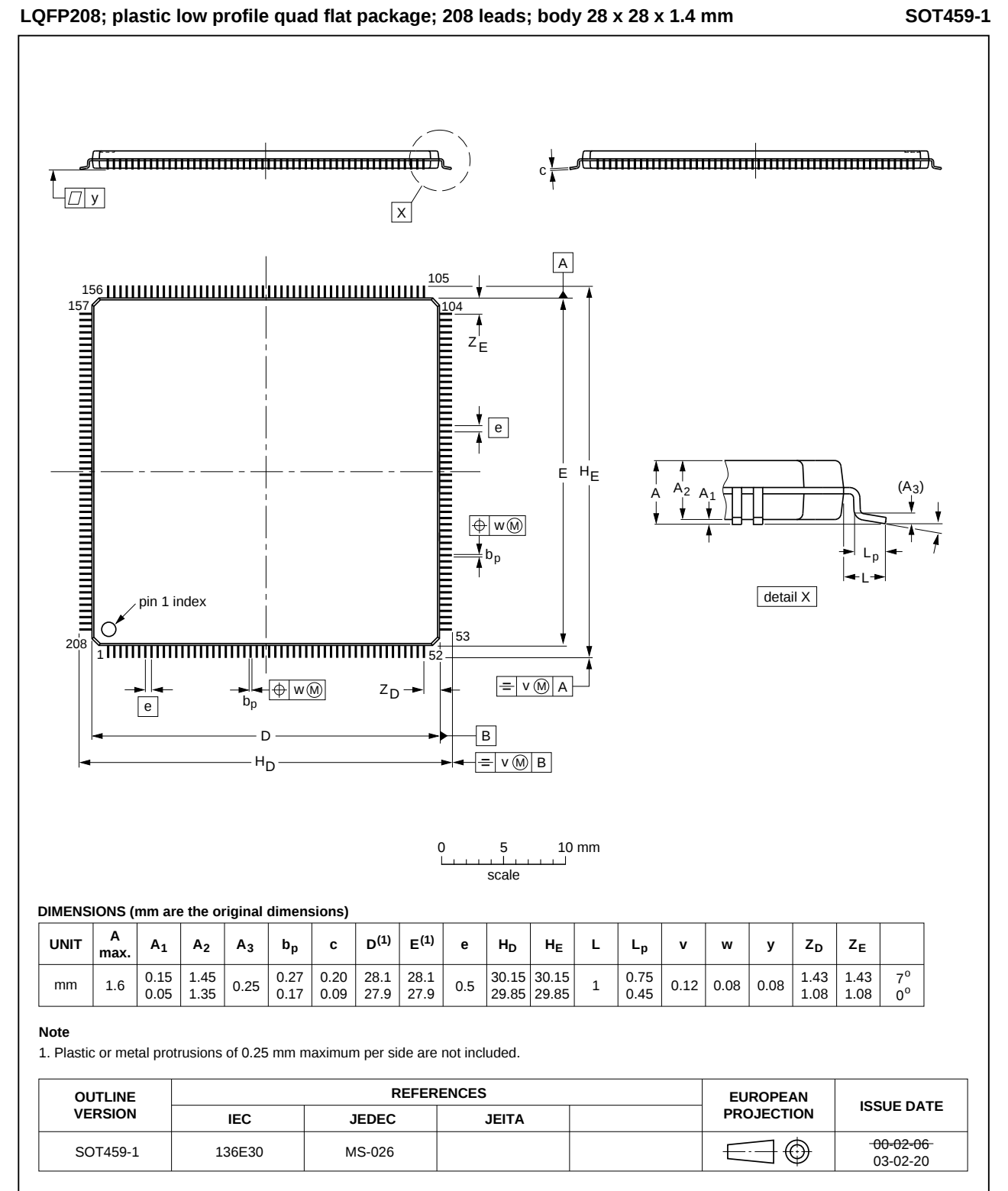
Fig 51. LQFP208 package
